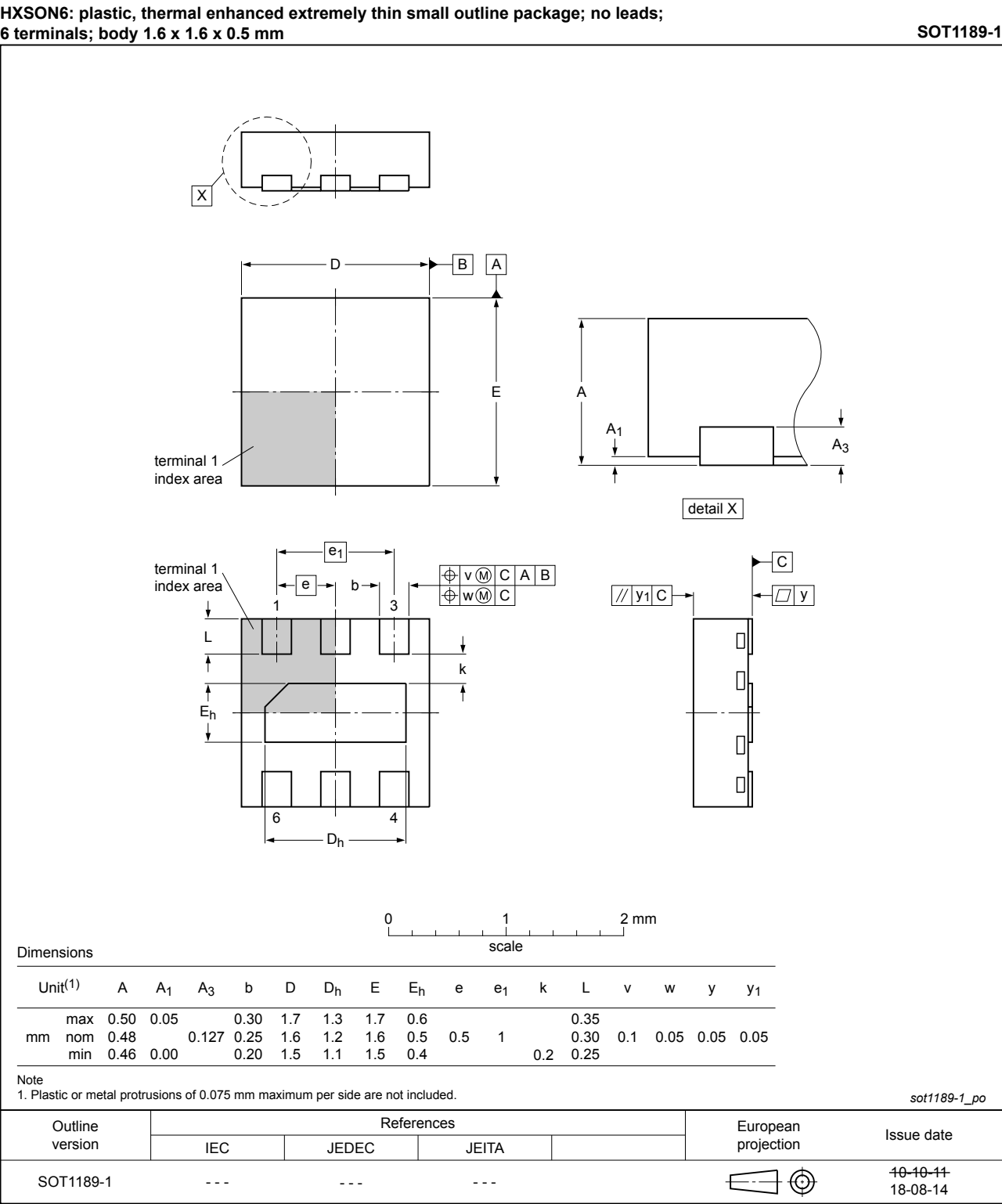
Figure 35. Package outline SOT1189-1 (HXSON6)
