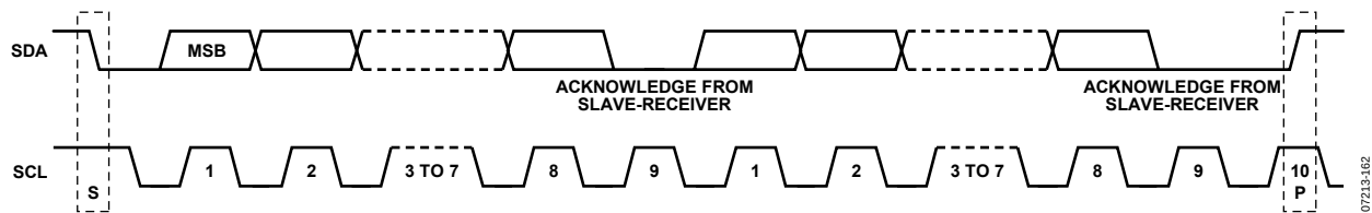
Figure 57. Acknowledge Bit
