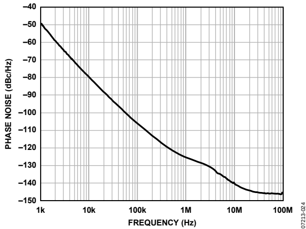
Figure 24. Internal VCO Phase Noise (Absolute), Direct-to-LVPECL @ 2750 MHz
