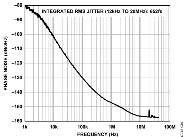
Figure 32. Phase Noise (Absolute) Clock Cleanup; Internal VCO @ 2.799 GHz; PFD = 120 kHz; LBW = 2.1 kHz; LVPECL Output = 155.52 MHz
