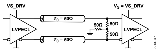
Figure 71. DC-Coupled 3.3 V LVPECL Y-Termination
