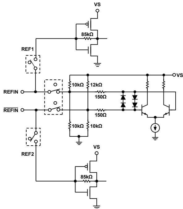
Figure 42. REF IN Equivalent Circuit for Non-XTAL Mode
