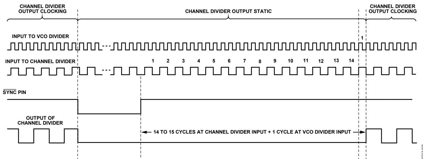
Figure 51. SYNC Timing Pipeline Delay When VCO Divider Is Used—CLK or VCO Is Input
