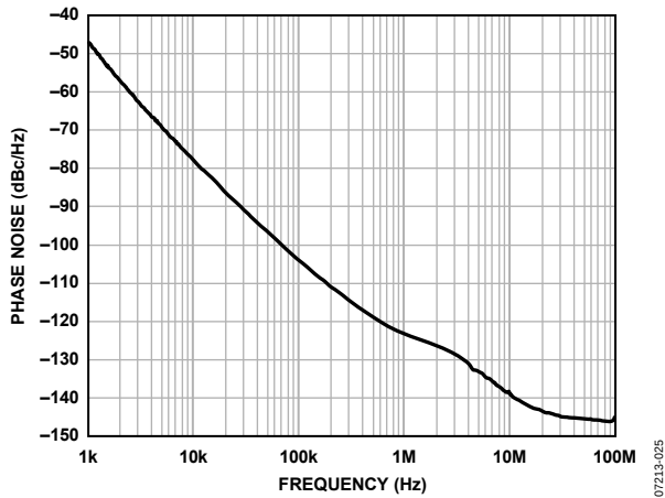
Figure 25. Internal VCO Phase Noise (Absolute), Direct-to-LVPECL @ 2950 MHz
