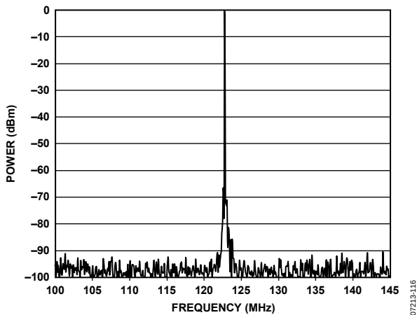
Figure 14. PFD/CP Spurs; 122.88 MHz; PFD = 15.36 MHz; LBW = 127 kHz; I_{CP} = 3.0 mA; f_{VCO} = 2703.4 MHz
