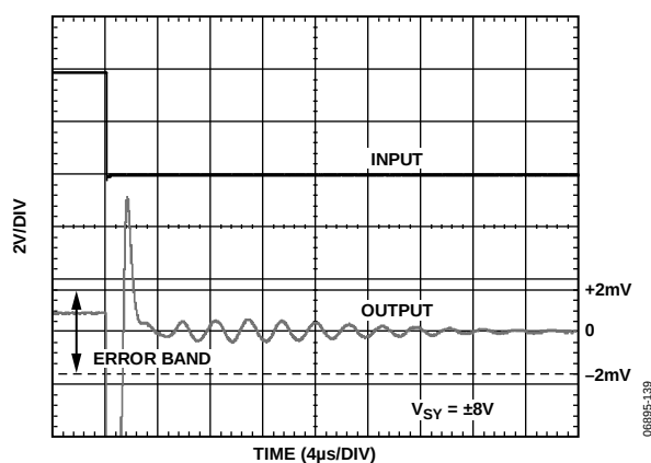
Figure 40. Negative Settling Time to 0.1%
