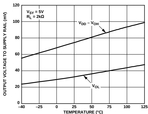
Figure 13. Output Voltage to Supply Rail vs. Temperature
