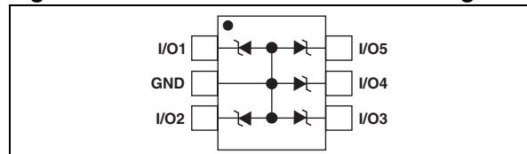
Figure 2. ESDA6V1-5P6 functional diagram
