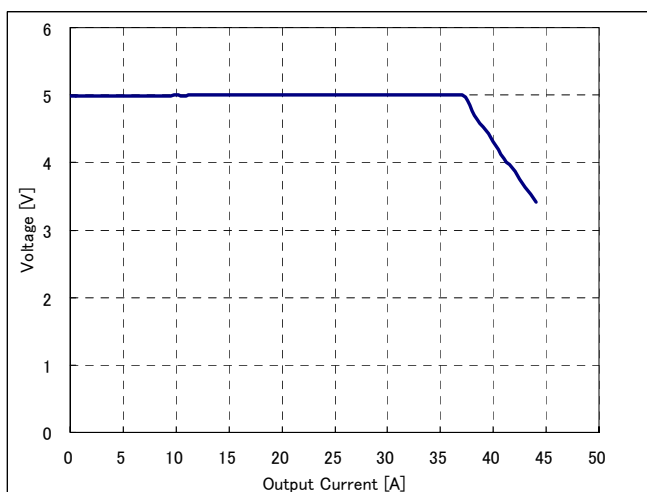
Fig-11: Output voltage vs. load current showing current limit point and converter shutdown point. ( V_{in} = 48\text{V} )
