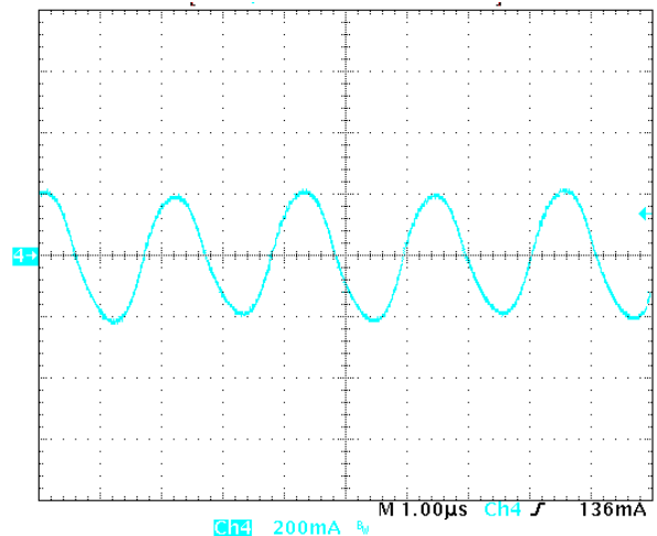
Fig-10: Input reflected ripple current, I_c (200mA/div), measured through 10\mu\text{H} at the source at full rated load current and V_{in}=48\text{V} . Time scale: 1\mu\text{s}/\text{div} .
