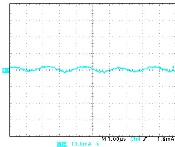
Fig-9: Input reflected ripple current, I_s (10mA/div), measured through 10\mu\text{H} at the source at full rated load current and V_{in}=48\text{V} . Time scale: 1\mu\text{s}/\text{div} .
