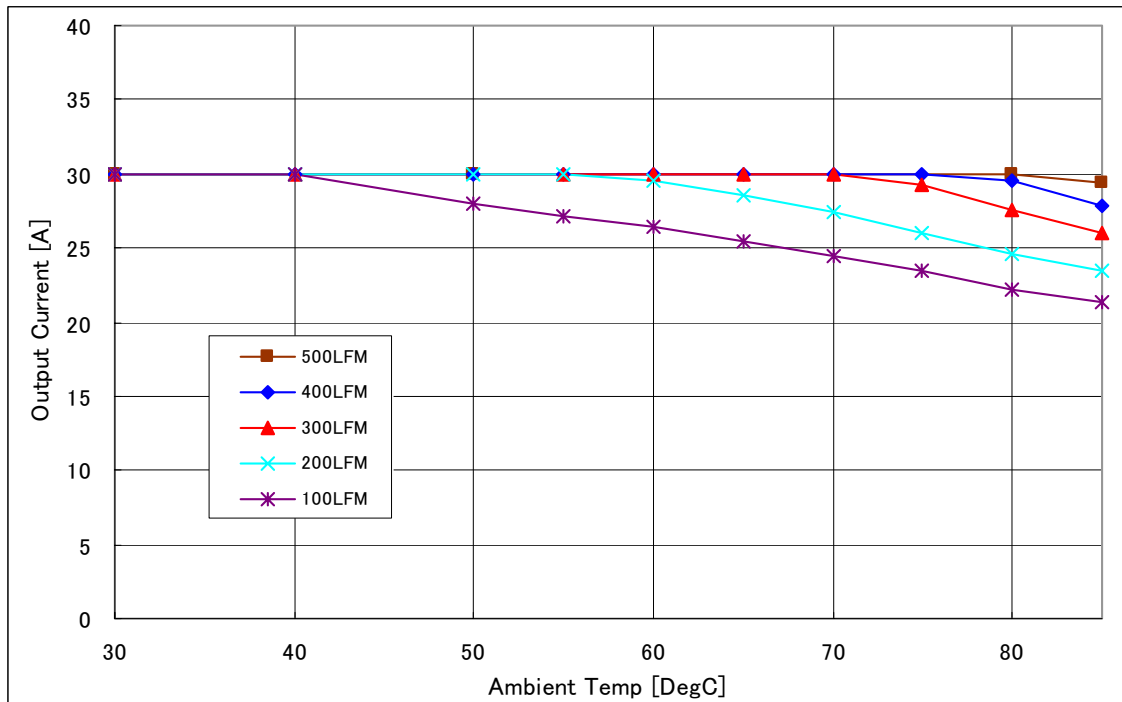
Fig-1: Available load current vs. ambient temperature and airflow rates for Vin=48V. Maximum component temperature \leq 125^{\circ}\text{C}
