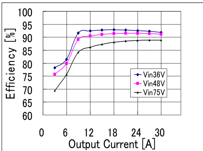
Fig-2: Efficiency vs. load current and input voltage for converter mounted horizontally with airflow from pin 3 to pin 1 at a rate of 200LFM (1.0m/s) and Ta=25°C.
