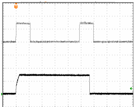
Fig-12: Load current (top trace, 50A/div, 20ms/div) into a 10\text{m}\Omega short circuit during restart, at V_{in} = 48\text{V} . Bottom trace (50A/div, 4ms/div) is an expansion of the top trace.
