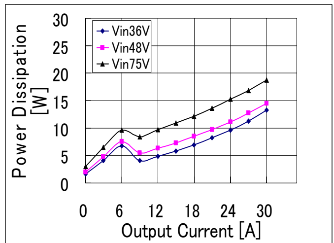
Fig-3: Power dissipation vs. load current and input voltage for converter mounted horizontally with airflow from pin 3 to pin 1 at a rate of 200LFM (1.0m/s) and Ta=25°C.
