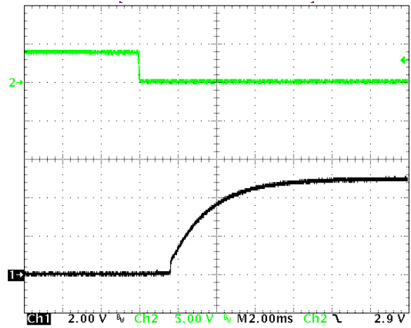
Fig-5: Turn-on transient at full rated load current (resistive) plus 10,000µF at V_{in}=48V , triggered via ON/OFF pin. Top trace: ON/OFF signal (5V/div). Bottom trace: output voltage (2V/div). Time scale: 2ms/div
