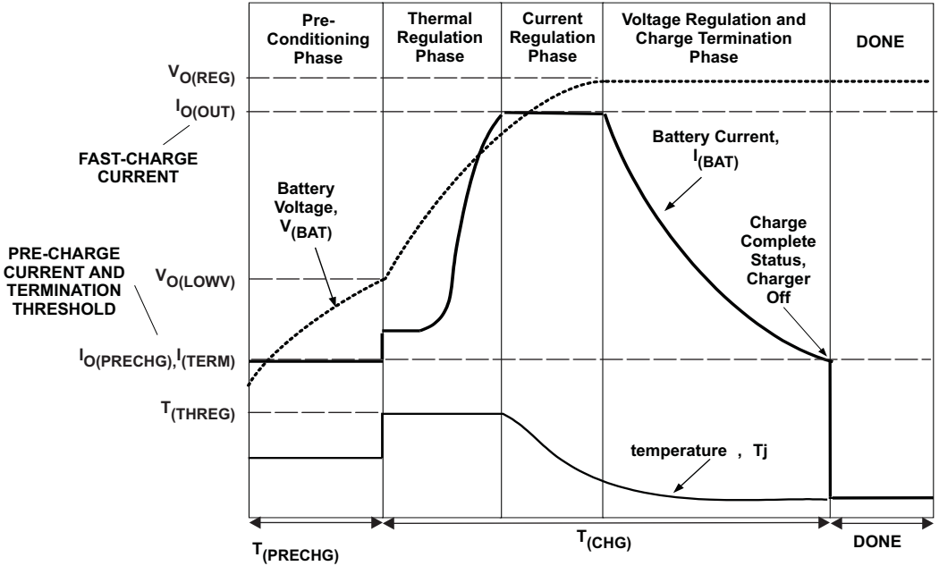
Figure 12. Charge Profile, Thermal Loop Active
