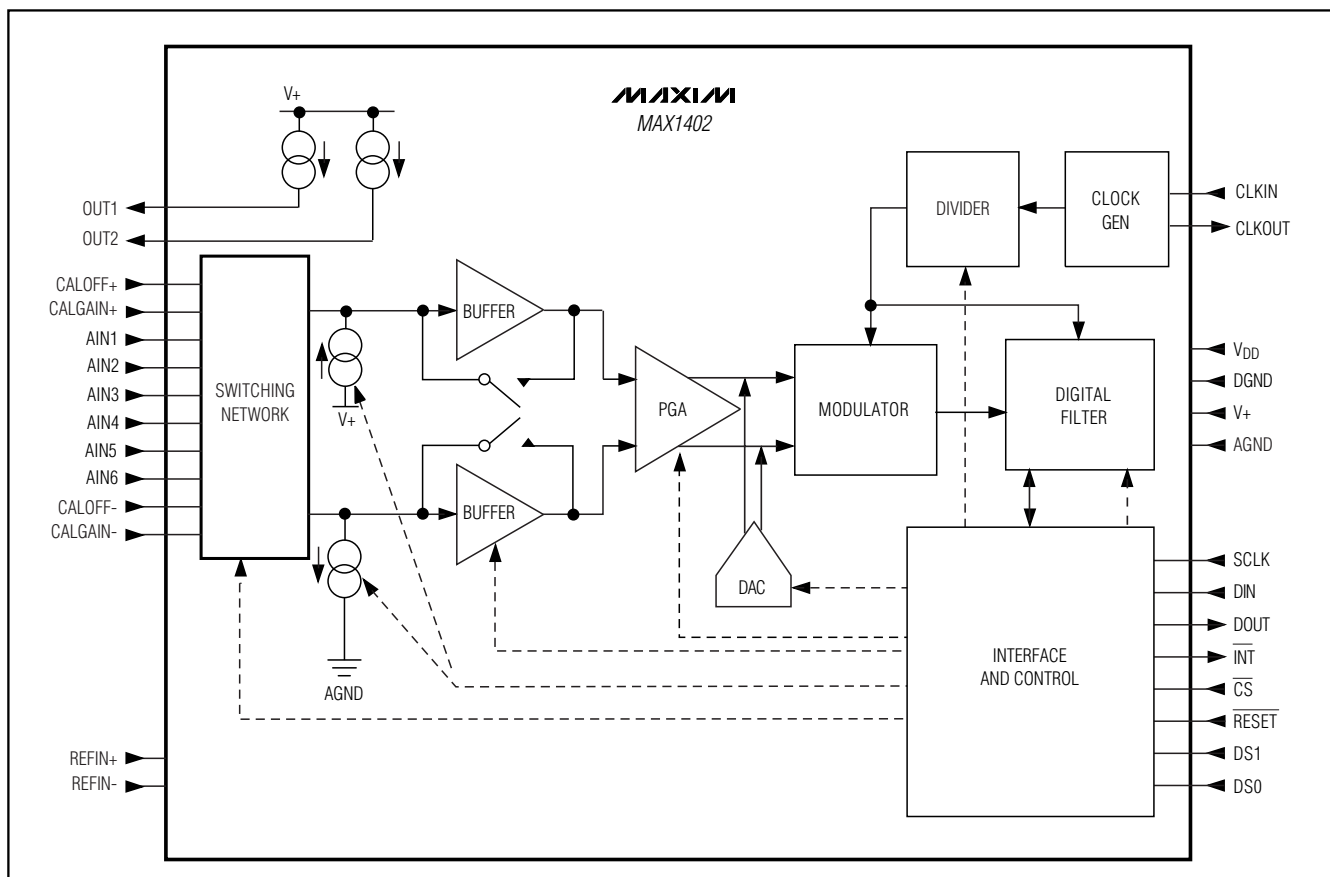
Figure 2. Functional Diagram
