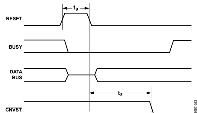
Figure 24. Reset Timing
