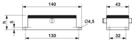
Dimensional drawing
