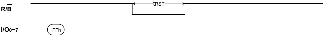
Figure 22. RESET Operation
