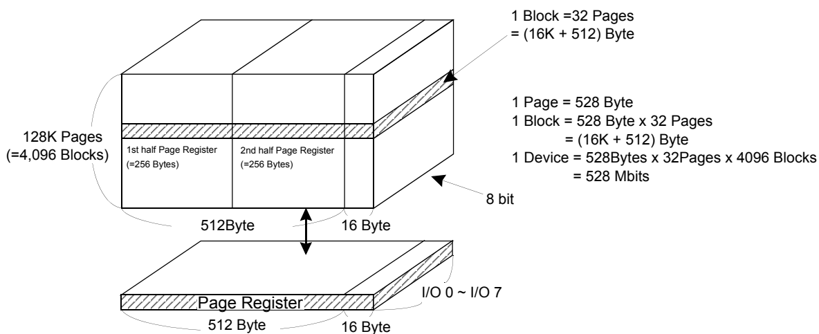
Figure 2-1. K9F1208X0B ARRAY ORGANIZATION
