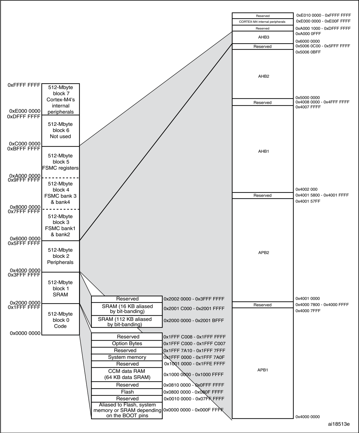
Figure 16. STM32F41x memory map
