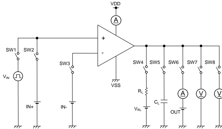
Figure 42. Test Circuit 2
