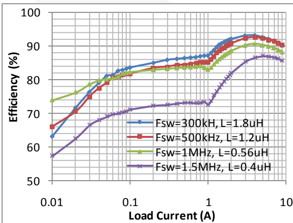
Figure 9. FAN2306MA Efficiency vs. Load Current with V_{IN}=12\text{ V} and V_{OUT}=1.2\text{ V}
