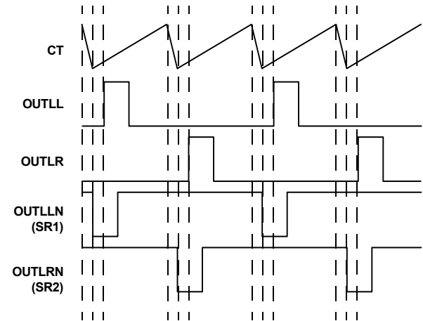
FIGURE 20. WAVEFORM TIMING WITH PWM OUTPUTS DELAYED, 0\text{V} < \text{VADJ} < 2.425\text{V}
