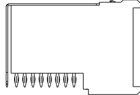
HM2R83PA8108N9 (top shielded only, 4 mm pitch)
