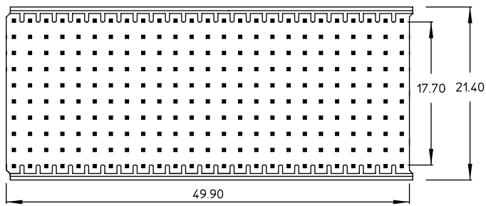
Standard loading patterns (seen from mating side)
