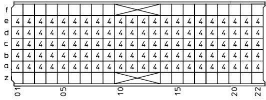
Standard loading patterns (seen from mating side)
