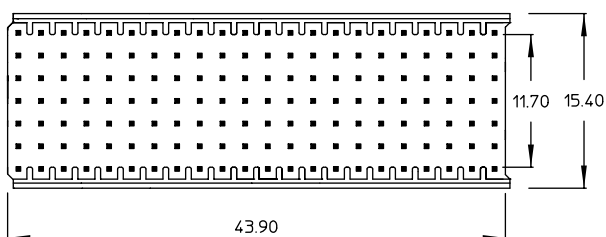
Standard loading patterns (seen from mating side)
