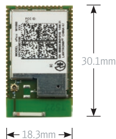
xPico Wi-Fi SMT XPCW1003100 (Actual Size)
