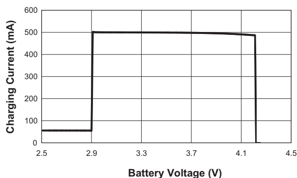
Charging Current vs. Battery Voltage (USBH; USBSET = 71.5kΩ)
