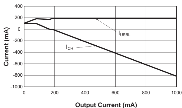
USB and Charging Current vs. Output Current (USBL; V_{BAT} = 3.6V )
