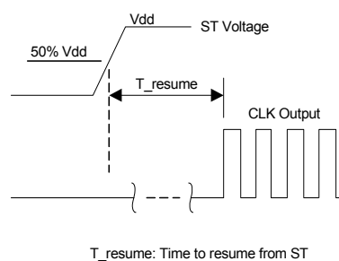
Figure 4. Standby Resume Timing (ST Mode Only)
