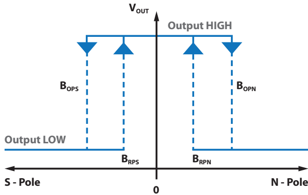
31.1 Omnipolar Magnetic Flux Response (Active Low Option)
