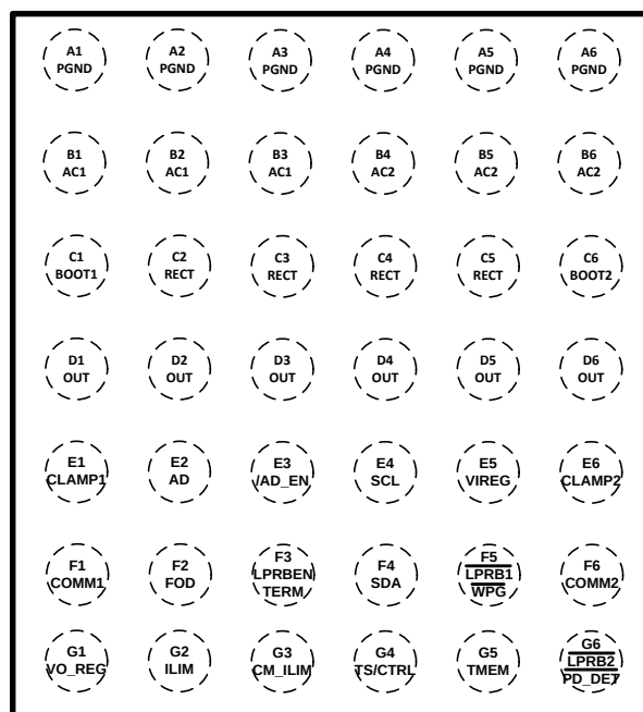
Pin Functions
