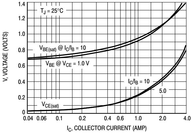
Figure 9. "On" Voltages
