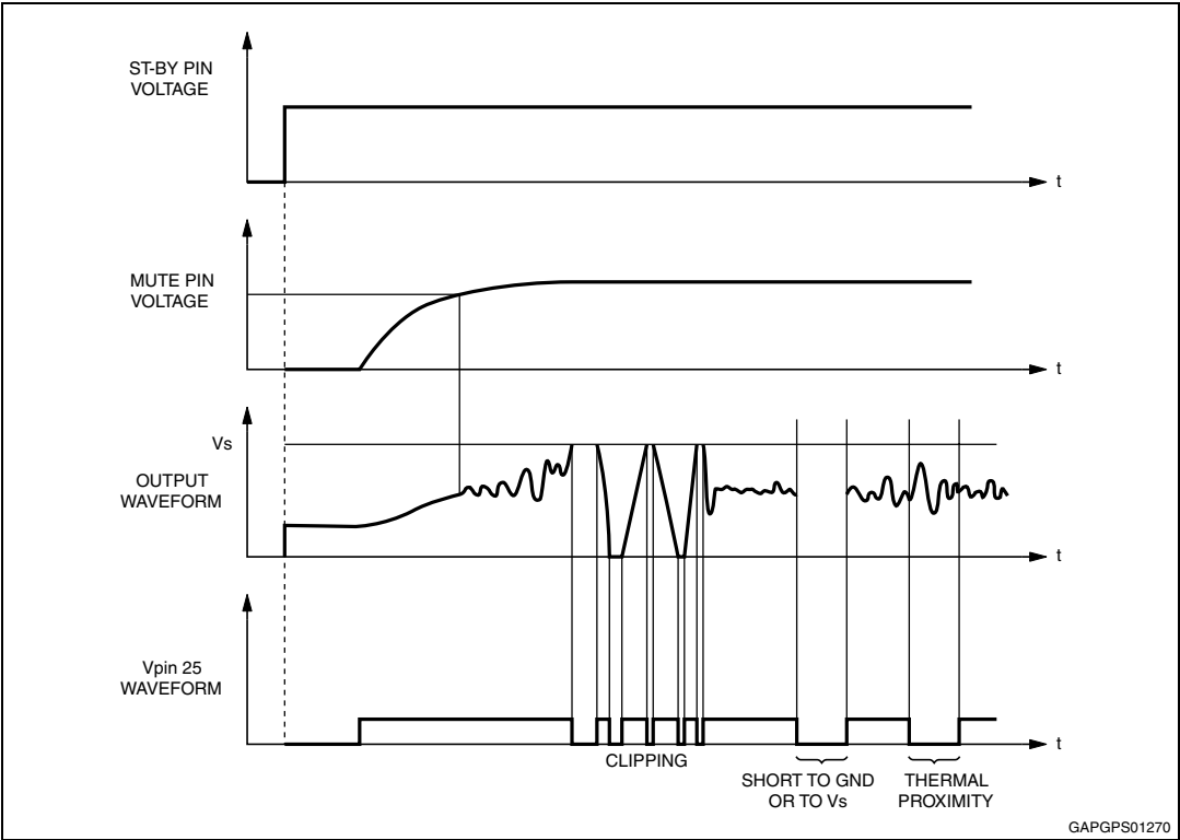
Figure 17. Diagnostics waveforms
