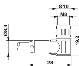
Socket M8 x 1, angled, shielded
