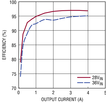
24V OUT Efficiency vs Output Current
