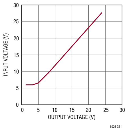
Minimum Required Input Running Voltage vs Output Voltage, I OUT = 5A
