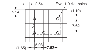
PCB Mounting Holes (Bottom View) Tolerance: \pm 0.1
