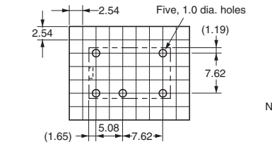
PCB Mounting Holes (Bottom View) Tolerance: \pm 0.1
