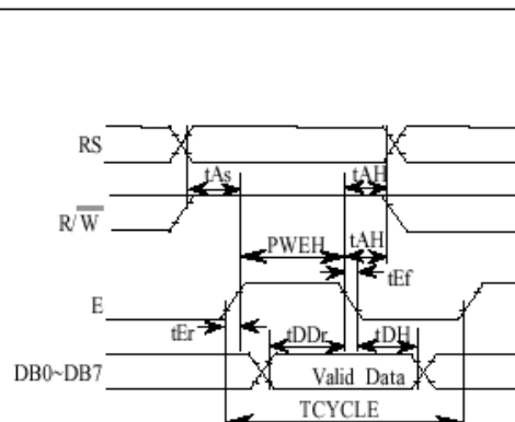
FIG 2. READ OPERATION
