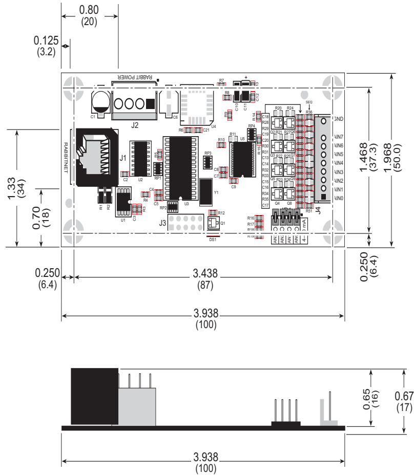
Figure 24. A/D Converter Card Dimensions
