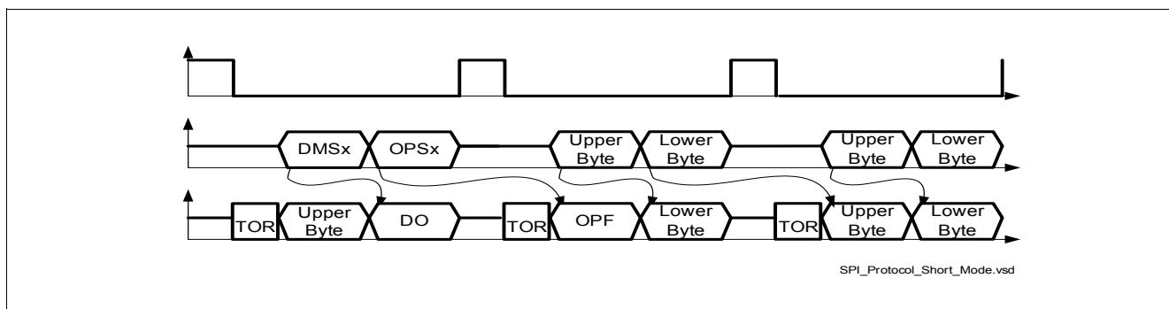
Figure 37 Data Transfer in Diagnosis and Compact Control
