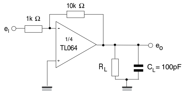
Figure 18. Gain-of-10 inverting amplifier
