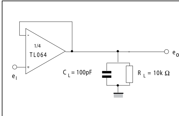
Figure 17. Voltage follower
