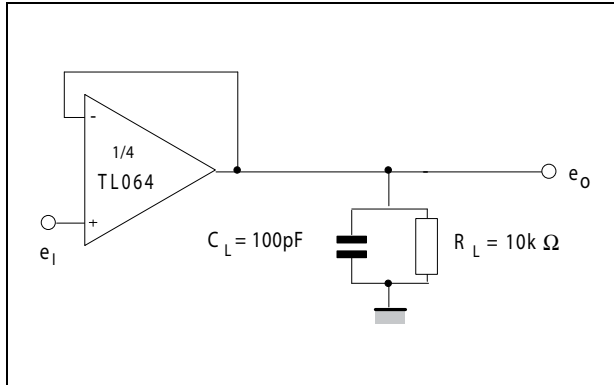
Figure 17. Voltage follower
