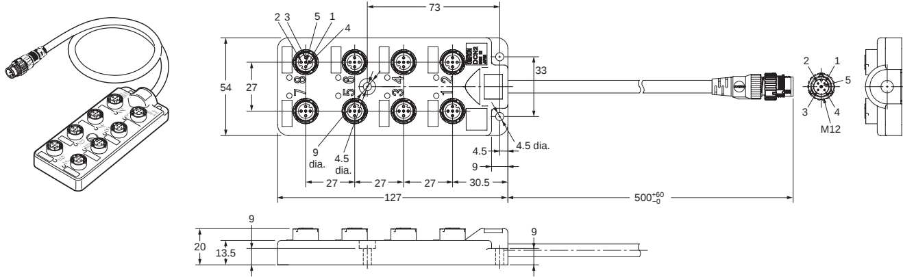
Connections Diagram
