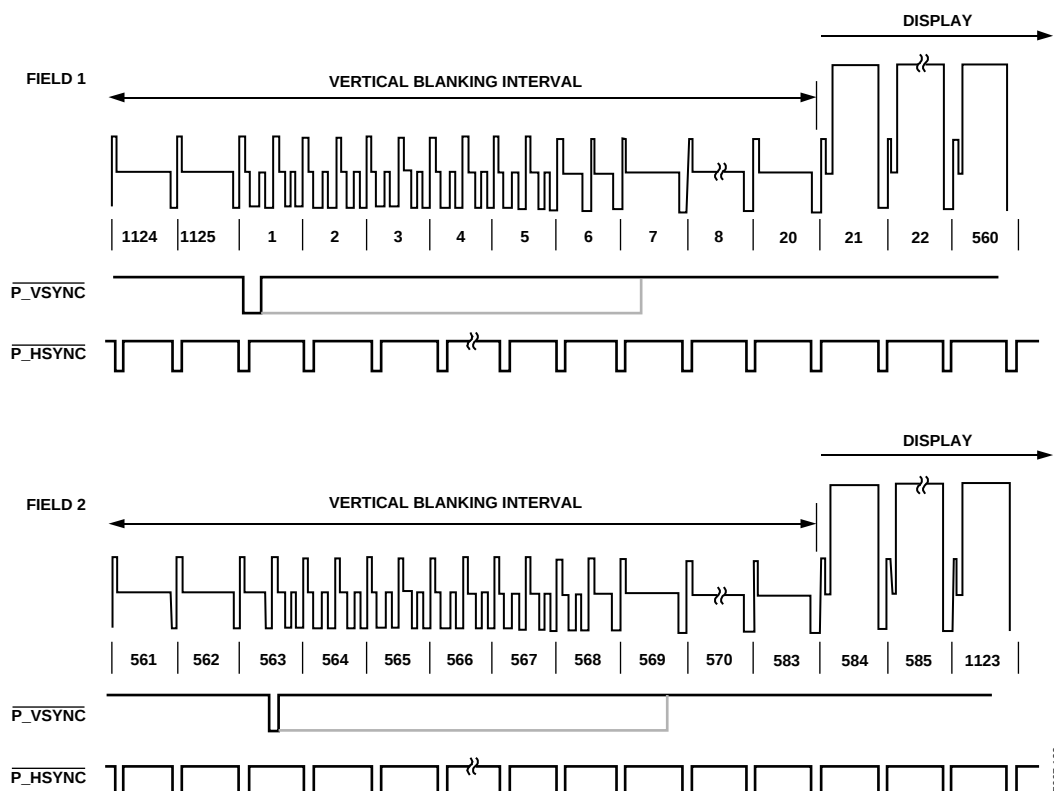
Figure 121. 1080i \overline{\text{HSYNC}} and \overline{\text{VSYNC}} Input Timing
