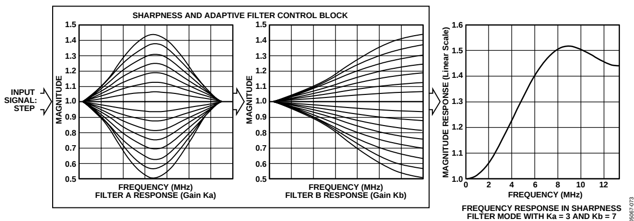
Figure 72. Sharpness and Adaptive Filter Control Block
