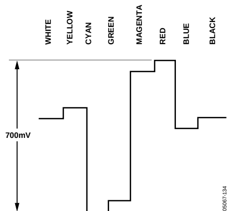
Figure 133. Pr Levels—PAL
