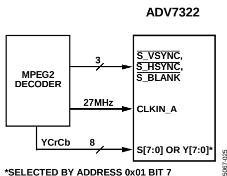
Figure 48. SD Only Input Mode
