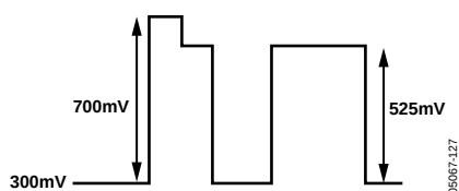
Figure 126. PS RGB Output Levels
