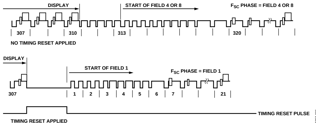
Figure 59. Timing Reset Timing Diagram
