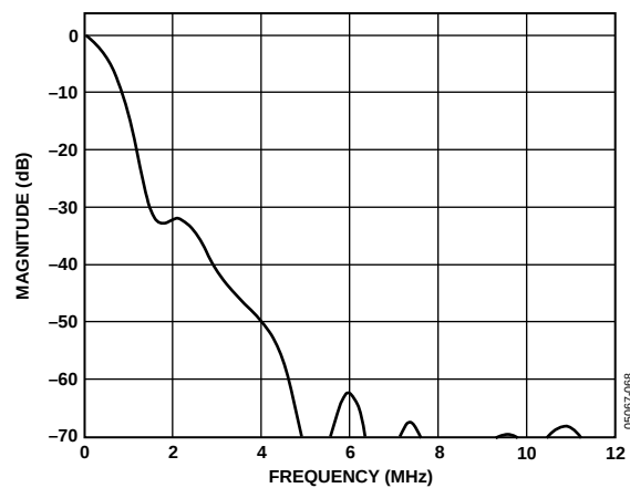
Figure 43. Chroma QCIF Low-Pass Filter
