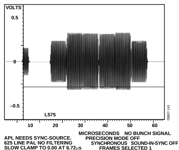
Figure 140. PAL Chroma
