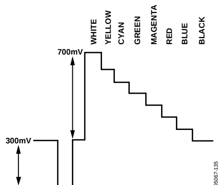
Figure 133. Pr Levels—PAL
