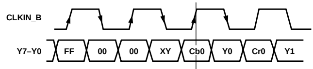
Figure 53. Input Sequence in PS Bit Interleaved Mode (EAV/SAV)
