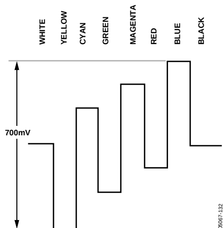
Figure 131. Pb Levels—PAL
