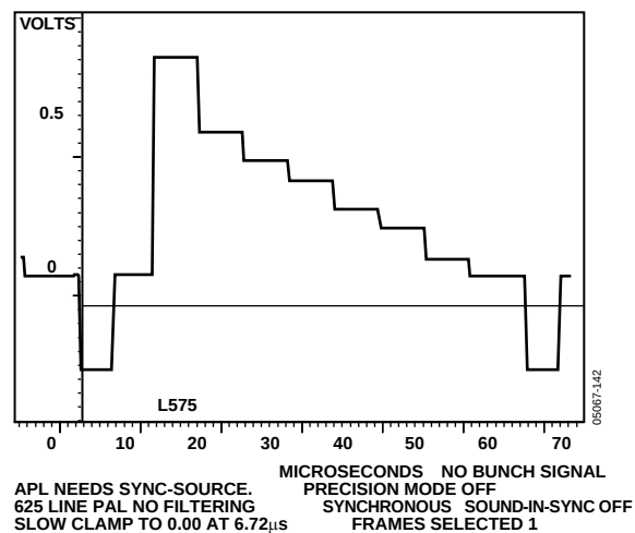
Figure 141. PAL Luma
