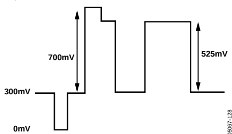
Figure 127. PS RGB Output Levels—RGB Sync Enabled
