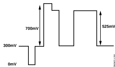
Figure 129. SD RGB Output Levels—RGB Sync Enabled
