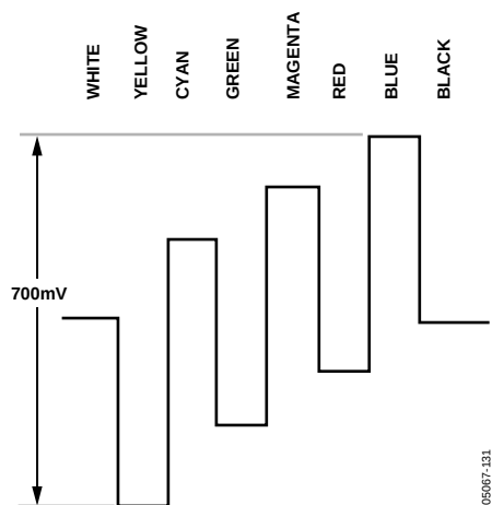
Figure 130. Pb Levels—NTSC
