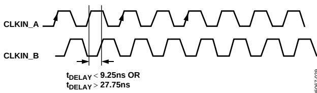
Figure 52. Clock Phase with Two Input Clocks
