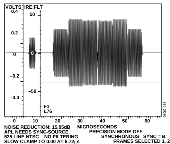
Figure 137. NTSC Chroma
