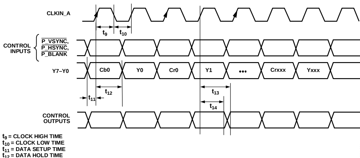
Figure 7. PS 4:2:2 8-Bit Interleaved at 54 MHz \overline{\text{HSYNC}}/\overline{\text{VSYNC}} Input Mode [Input Mode 111]
