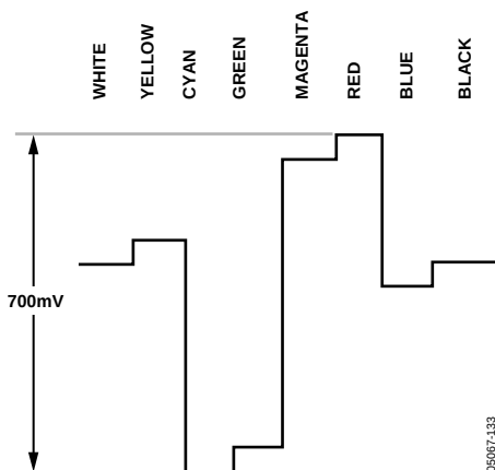
Figure 131. Pb Levels—PAL
