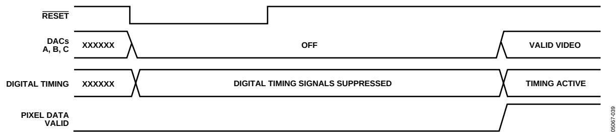
Figure 62. RESET Timing Sequence
