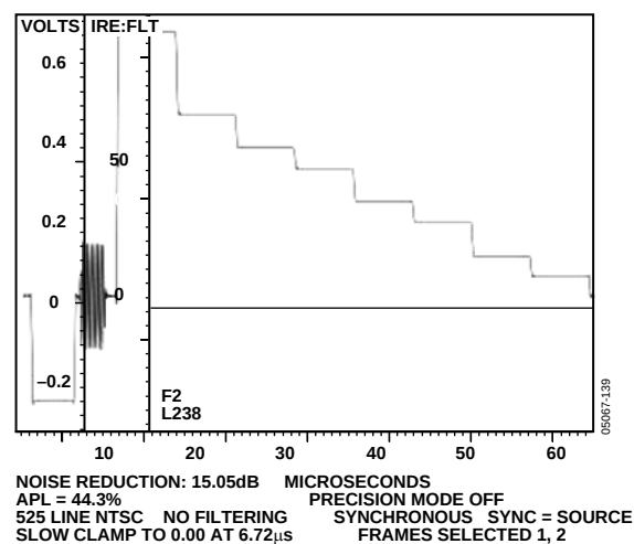
Figure 138. NTSC Luma
