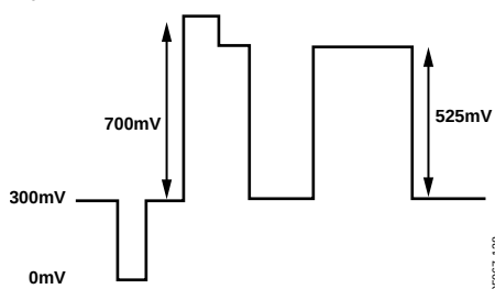
Figure 127. PS RGB Output Levels—RGB Sync Enabled
