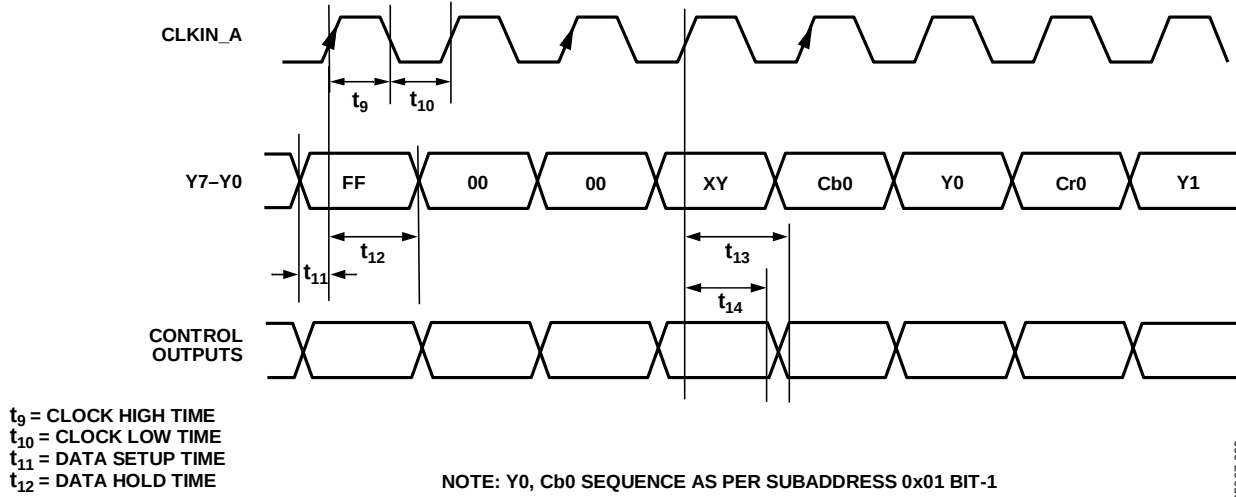
Figure 9. PS Only 4:2:2 8-Bit Interleaved at 54 MHz EAV/SAV Input Mode [Input Mode 111]
