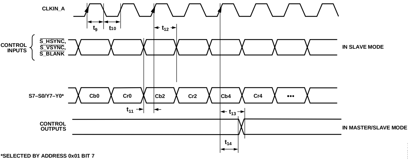
Figure 13. 8-Bit SD Only Pixel Input Mode [Input Mode 000]
