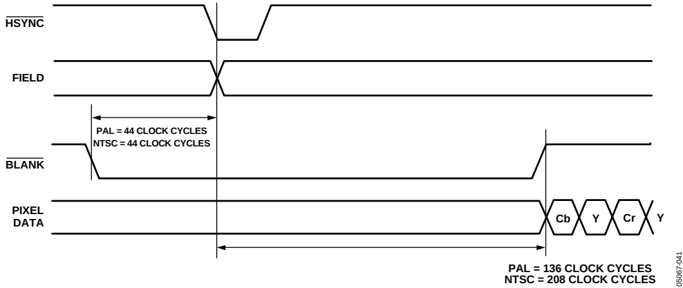
Figure 64. Active Pixel Timing
