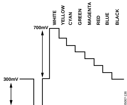
Figure 134. Y Levels—NTSC
