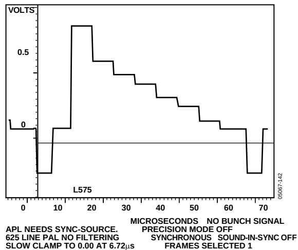
Figure 141. PAL Luma
