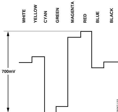
Figure 131. Pb Levels—PAL
