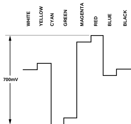
Figure 133. Pr Levels—PAL
