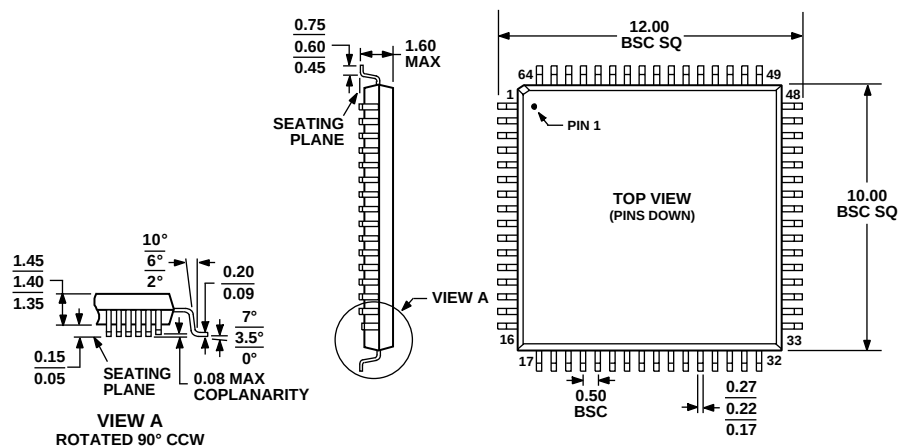
Figure 148. 64-Lead Low Profile Quad Flat Package [LQFP] (ST-64-2) Dimensions shown in millimeters
