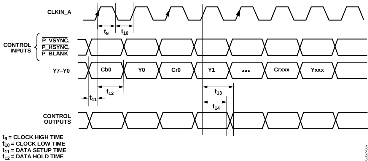
Figure 7. PS 4:2:2 8-Bit Interleaved at 54 MHz \overline{\text{HSYNC}}/\overline{\text{VSYNC}} Input Mode [Input Mode 111]
