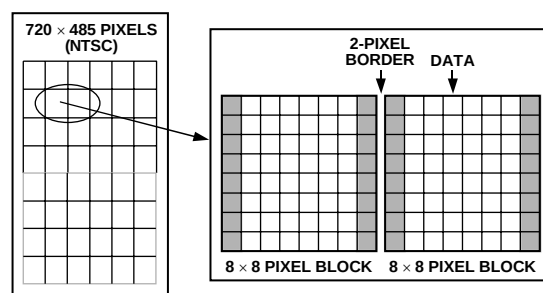
Figure 79. DNR Border Area
