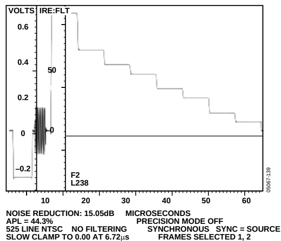
Figure 138. NTSC Luma
