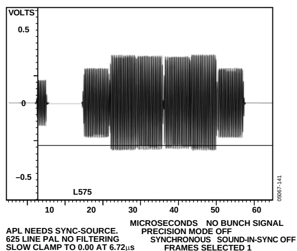
Figure 140. PAL Chroma
