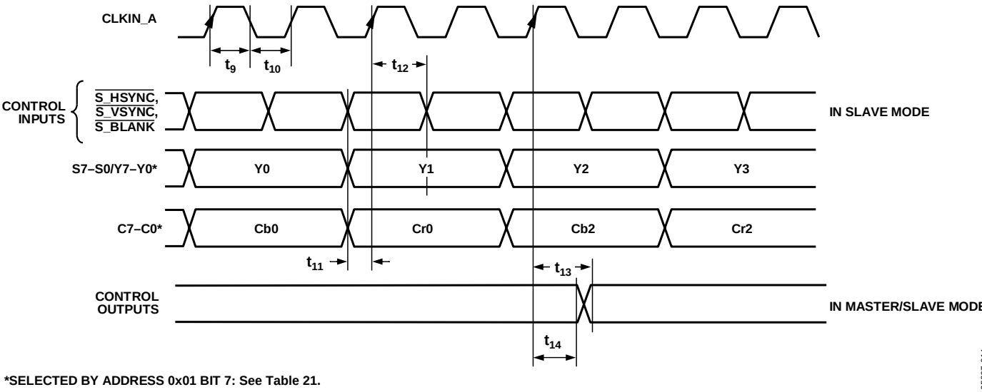
Figure 14. 16-Bit SD Only Pixel Input Mode [Input Mode 000]
