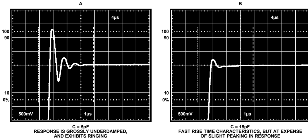
Figure 49. Effect of Altering Compensation from Circuit in Figure 47—PM7545 CMOS DAC with 1/2 OP249, Unipolar Operation; Critically Damped Response Is Obtained with C \approx 33 pF
