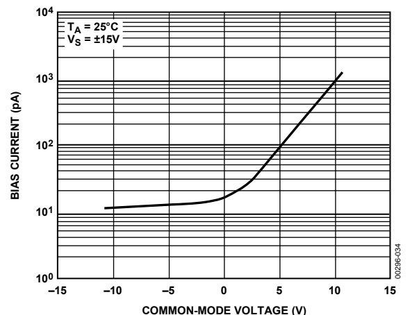
Figure 34. Bias Current vs. Common-Mode Voltage
