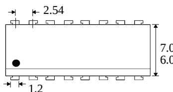
TLP521-4
