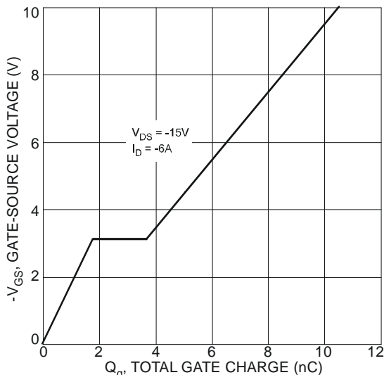
Figure 23. Gate-Charge Characteristics
