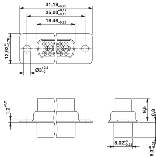
Dimensioned drawing
