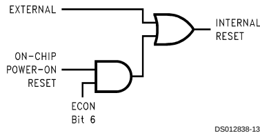
FIGURE 8. Reset Logic
