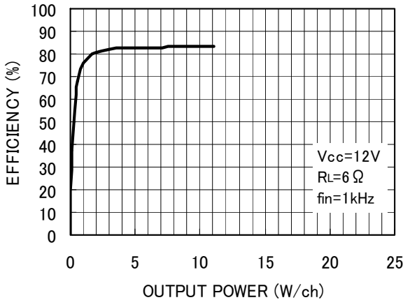
Fig. 20 Efficiency - Output power
