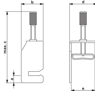
Dimensioned drawing
