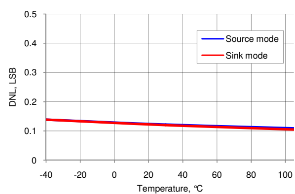
Figure 11-52. IDAC DNL vs Temperature, Range = 255 \mu A, Fast Mode
