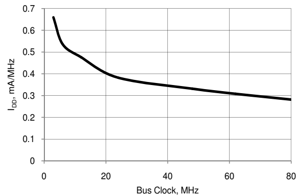
Figure 11-2. I_{DD} vs Frequency at 25^\circ\text{C}
