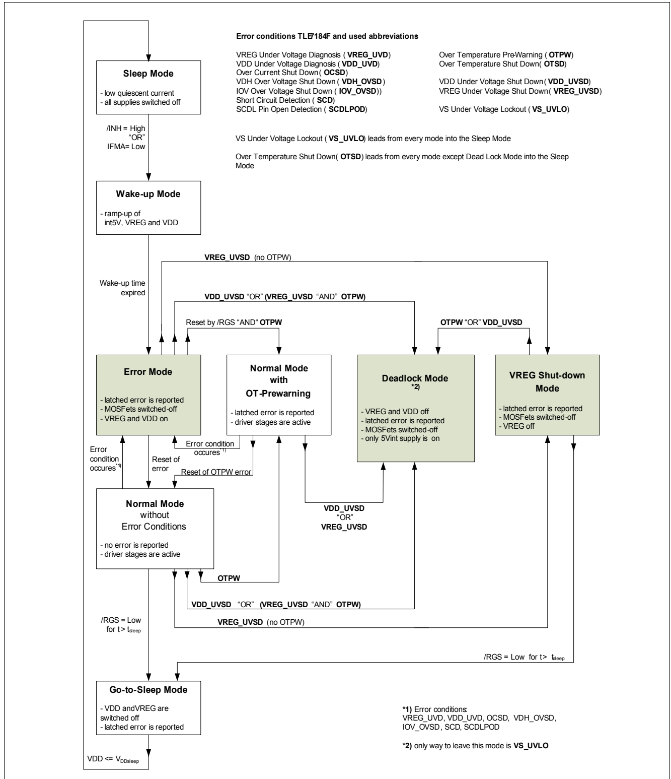
Figure 10 State diagram TLE7186F
