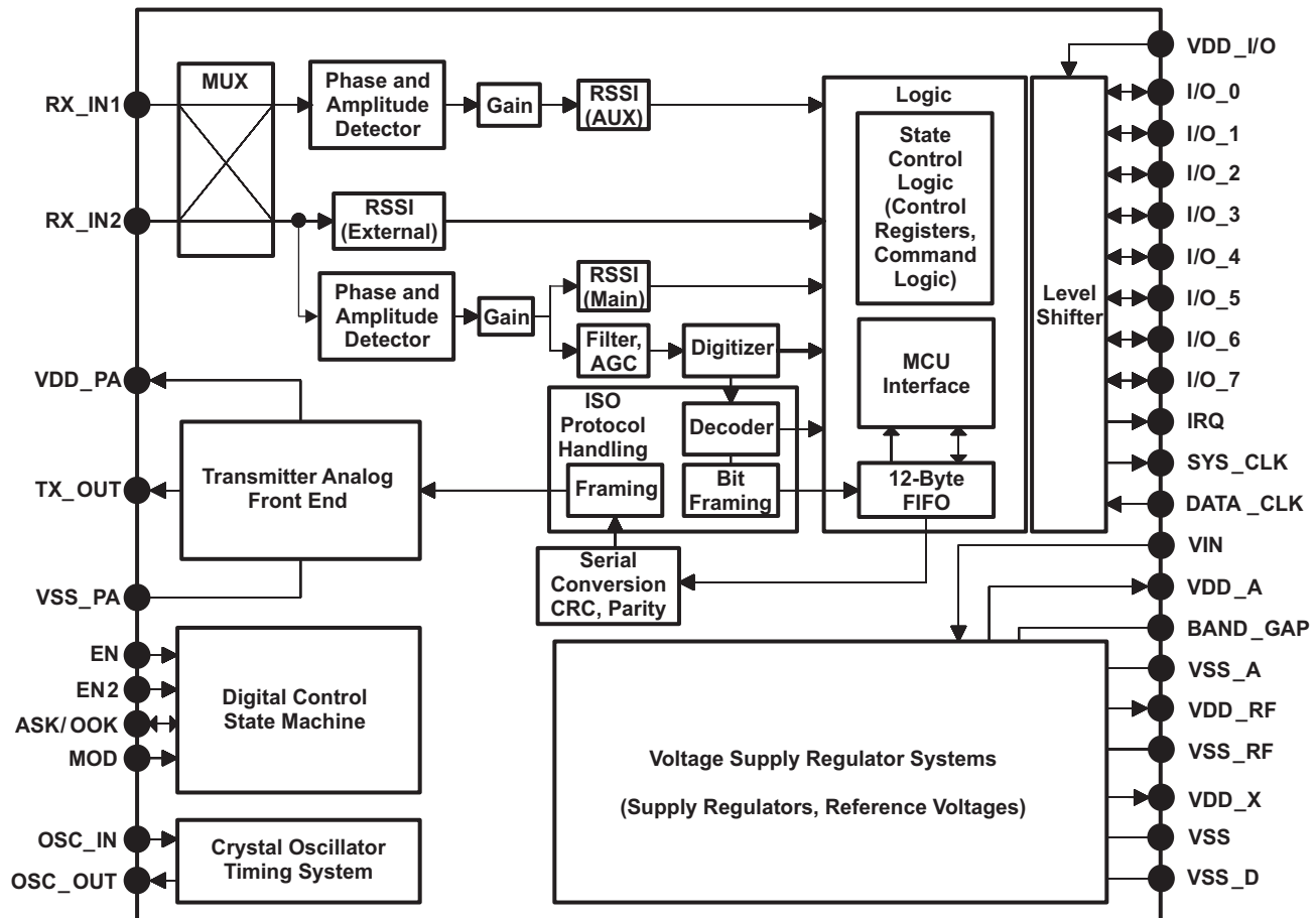
Figure 1-1. Block Diagram
