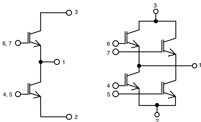
Functional Diagram
