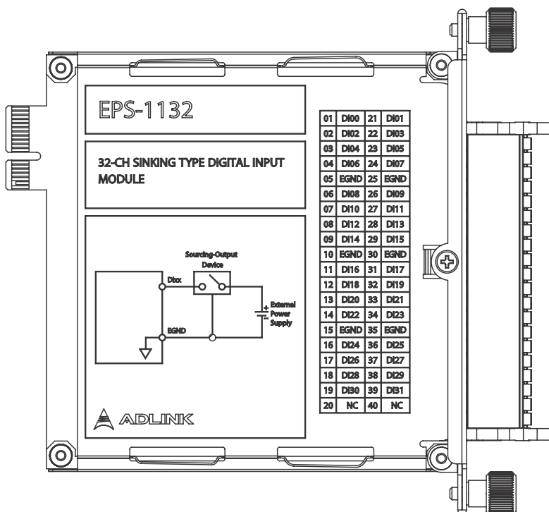
Figure 3-2: EPS-1132 Schematic
