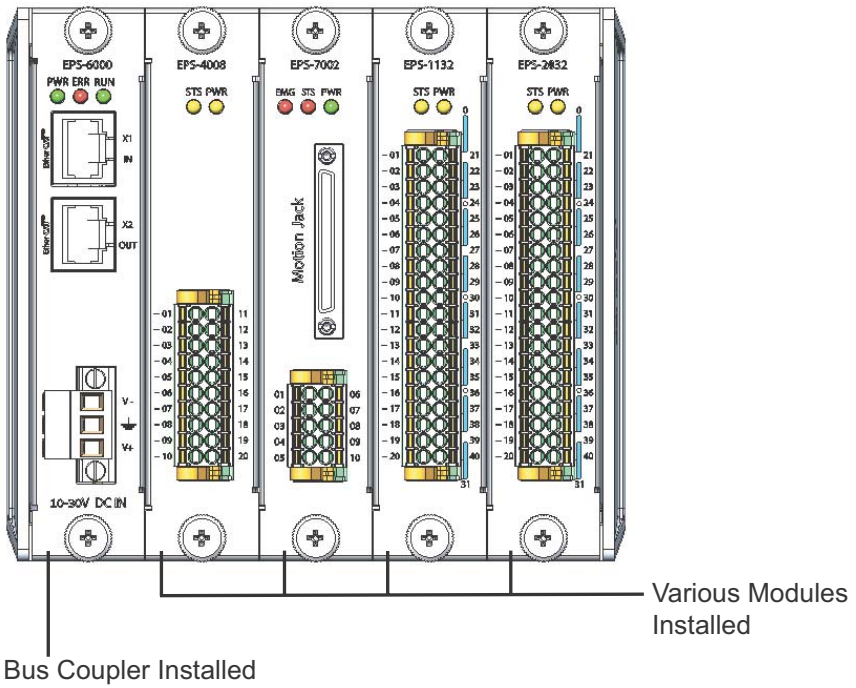
Figure 1-5: EPS System w/ Modules Installed
