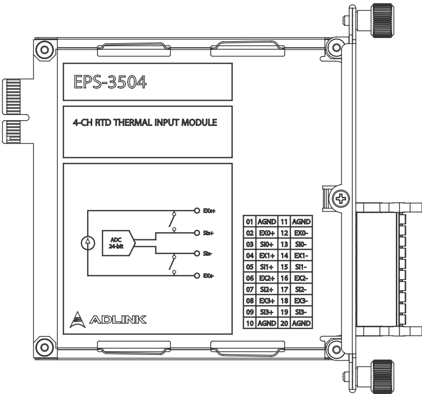
Figure 3-8: EPS-3504 Schematic
