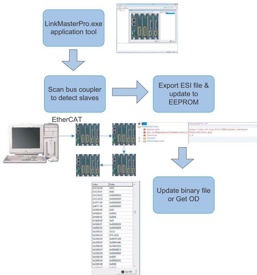
Figure A-1: LinkMasterPro™ Operational Overview
