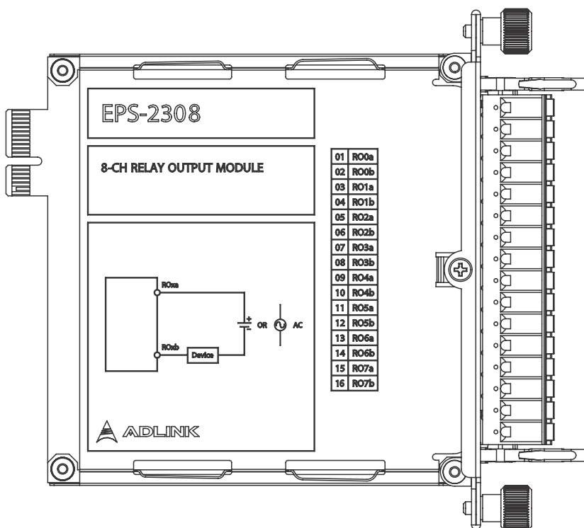
Figure 3-5: EPS-2308 Schematic
