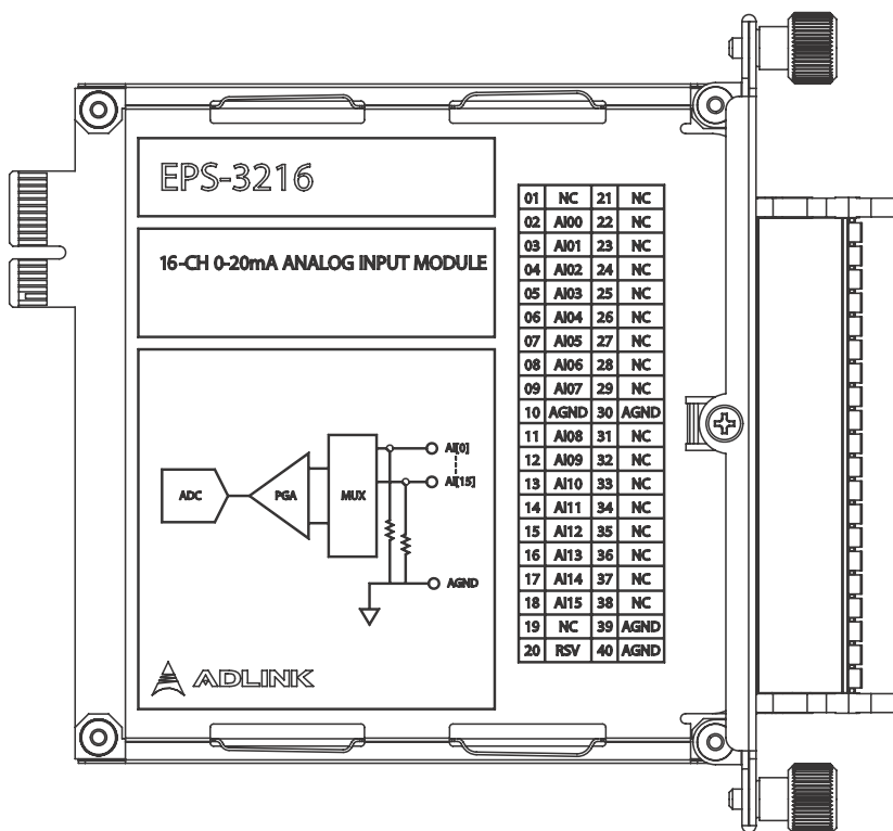
Figure 3-7: EPS-3216 Schematic
