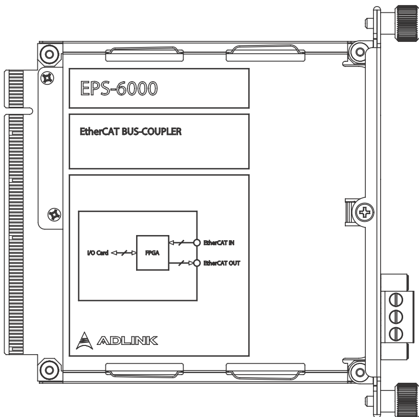
Figure 3-10: EPS-6000 Schematic
