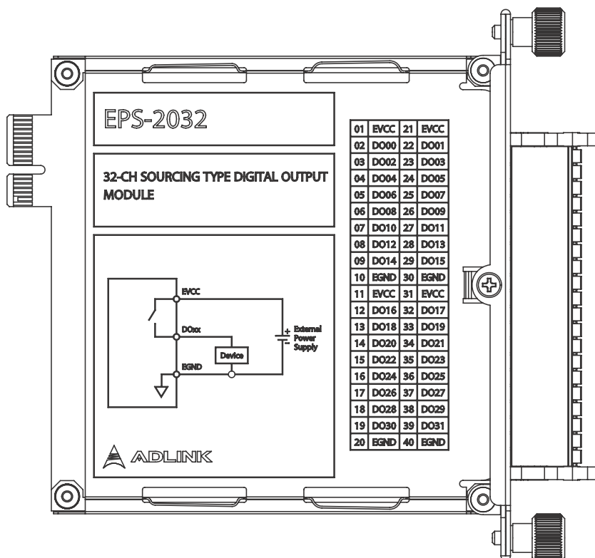
Figure 3-3: EPS-2032 Schematic
