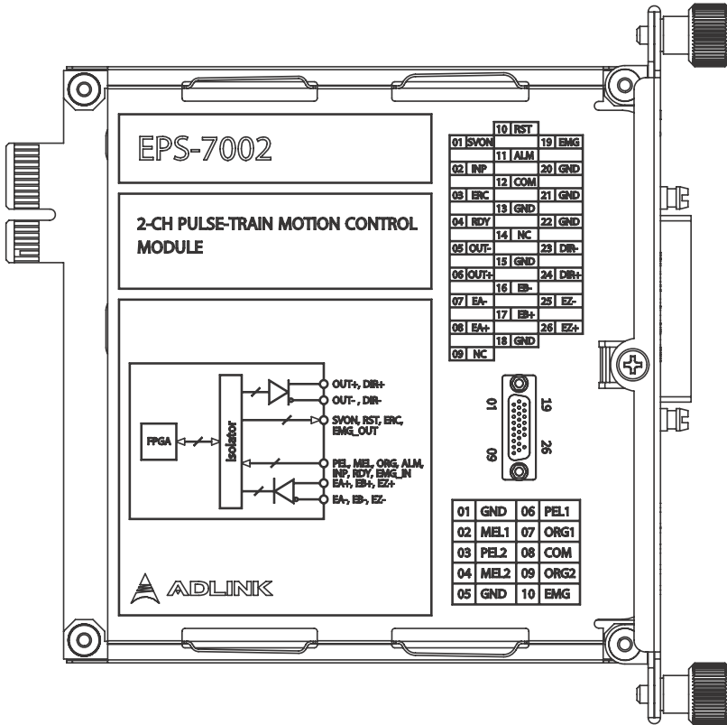
Figure 3-11: EPS-7002 Schematic
