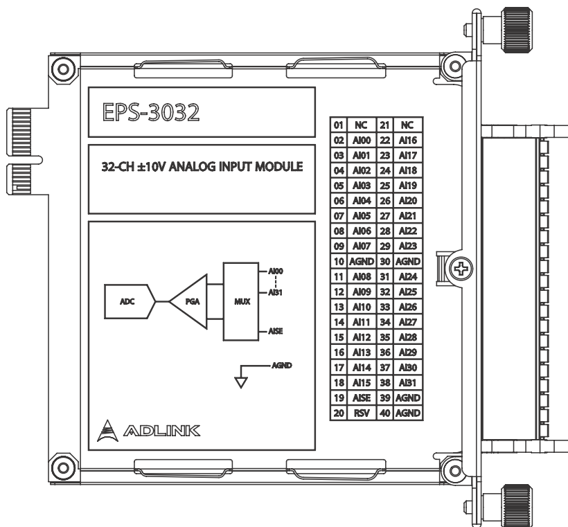
Figure 3-6: EPS-3032 Schematic
