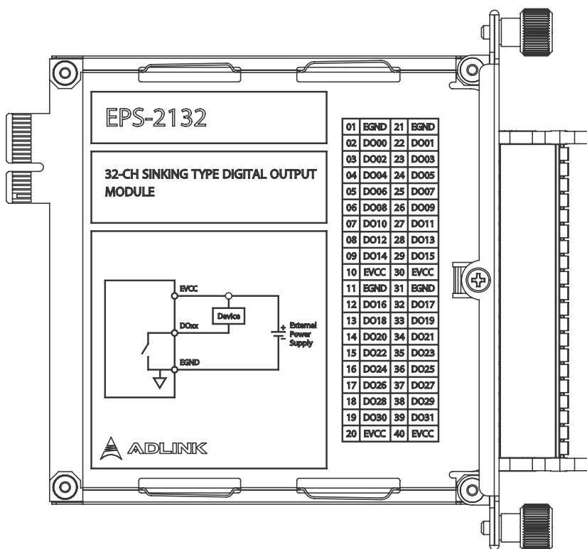
Figure 3-4: EPS-2132 Schematic
